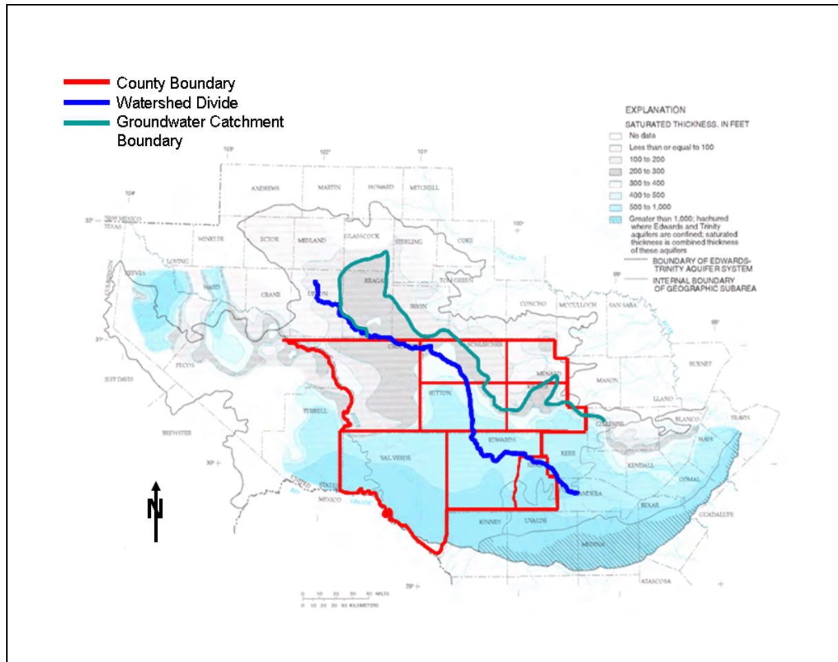
Figure 14. Contour map of the saturated thickness of the Edwards-Trinity Aquifer with the surface-water divide separating the Rio Grande watershed from the Colorado River watershed (blue line) and the extent of groundwater piracy estimated using the 200-ft saturated thickness contour of the Edwards-Trinity Aquifer (green line).
