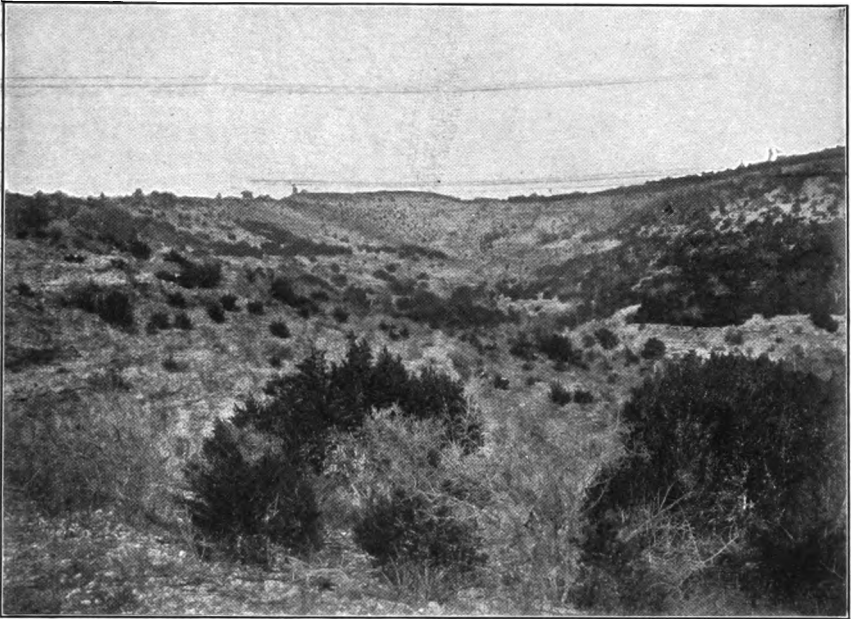
FIG. 1.—“SOUTH GORGE” AT ITS HEAD UNDER LONE TREE HILL, NEAR AUSTIN. The slopes have been denuded of timber. The run-off water after heavy rainfall is very violent.
