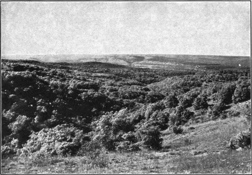
FIG. 1.—CHARACTERISTIC VIEW OF THE EDWARDS PLATEAU FOREST, ON THE COLORADO RIVER, 10 MILES ABOVE AUSTIN.
